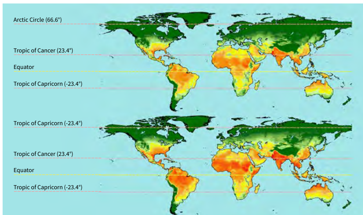
Fig. 1.1: Monthly mean WBGT in the shade during the hottest month of the year around the world (0.5° × 0.5° grid cells) for the end of the century (2071–2099) if aggressive measures are taken to reduce greenhouse gas emissions to keep the global mean temperature at a maximum 1.5°C increase with a decreasing trend in the second half of this century (RCP2.6, top panel), or if countries implement existing national policies (RCP6.0, bottom panel). Source: International Labour Organization, Working on a warmer planet (5)
