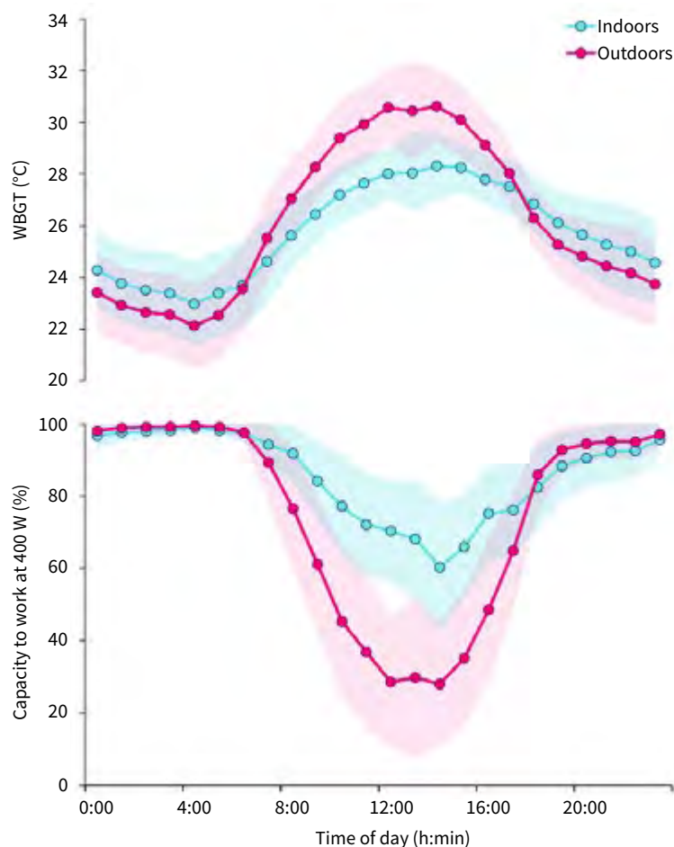
Fig. 2.8: Outdoor and indoor WBGT (top graph) and resulting ability to perform work (bottom graph) at a moderate to heavy pace (percentage of time that an individual can work at 400 W metabolic rate) during different hours of the day in Delhi, India, in May 1999. Lines indicate the monthly average and shaded areas indicate monthly standard deviation. Source: Graphs based on previously published data (25); estimates based on hourly weather data from the United States National Oceanic and Atmospheric Administration database
