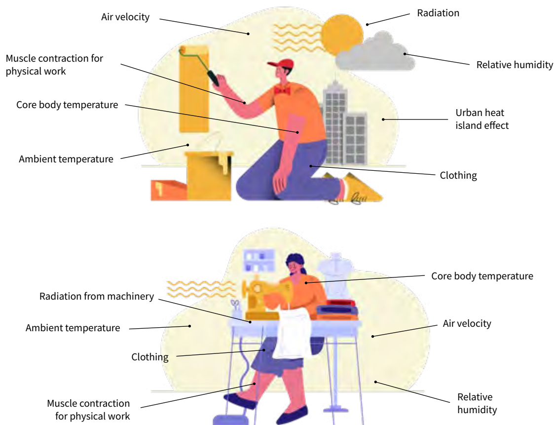
Fig. 1.2a: Illustration of the interaction of different occupational factors that can increase heat stress. Work demands dictate the internal metabolic rate, which is the major source of heat gain. Environmental factors and clothing determine the remaining avenues of heat exchange. The asterisk indicates that conduction and convection can lead to heat gain or loss; under most conditions, these are relatively minor avenues of heat exchange
